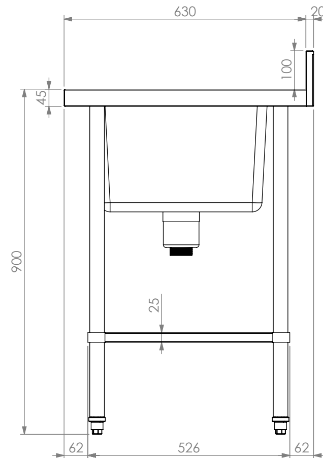
SIDE ELEVATION
